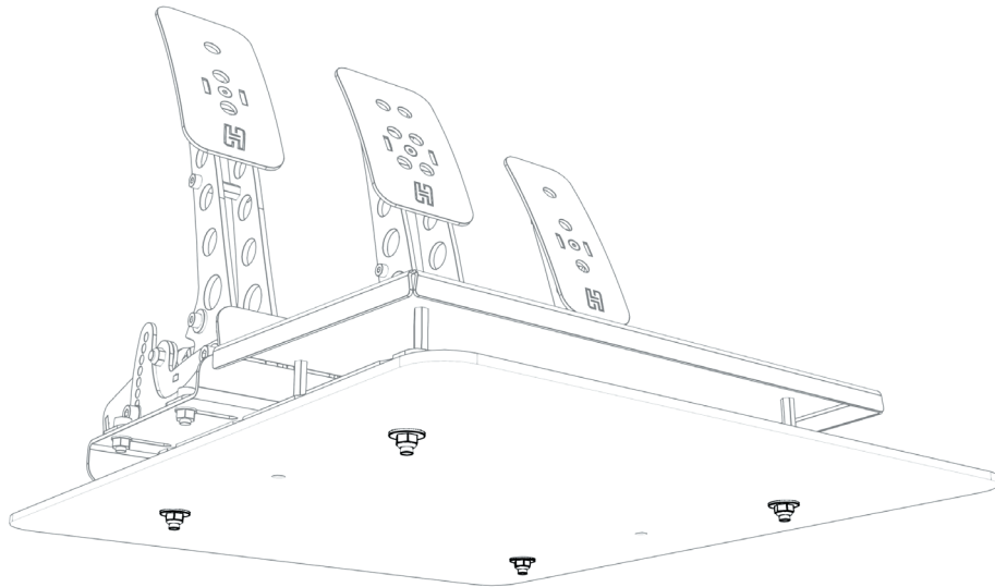
Mounting the baseplate - most solid mount (viewed from below).
