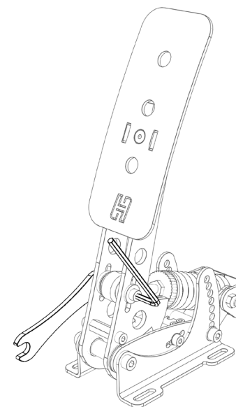
Step 1: Loosen nut on the adjustment bolt.
